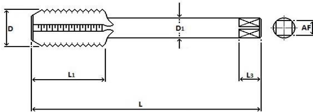
ISO 529 TAP BLANK DIMENSIONS FOR THREADS OVER 1" (25.4mm) DIAMETER
