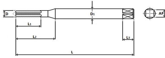
ISO 529 TAP BLANK DIMENSIONS FOR THREADS UP TO 1/8" (3mm) DIAMETER
